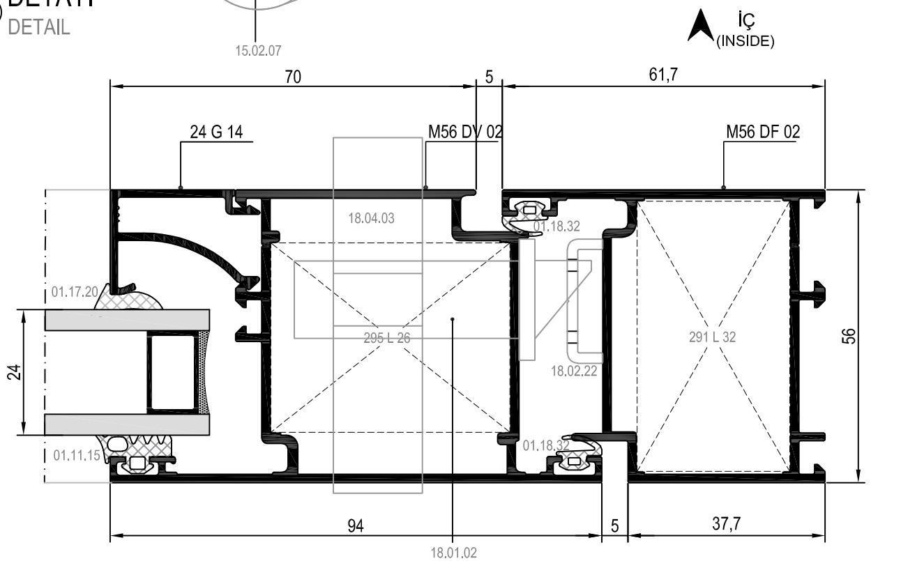
32 DETAYI DETAIL
