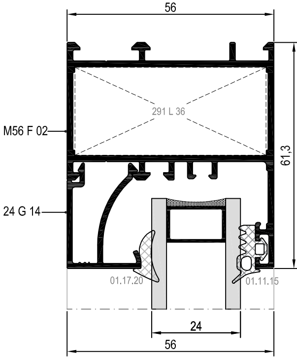
28 DETAYI DETAIL
