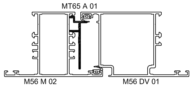
İÇE AÇILIM HEMYÜZ KAPI INWARD OPENING FLUSH DOOR
