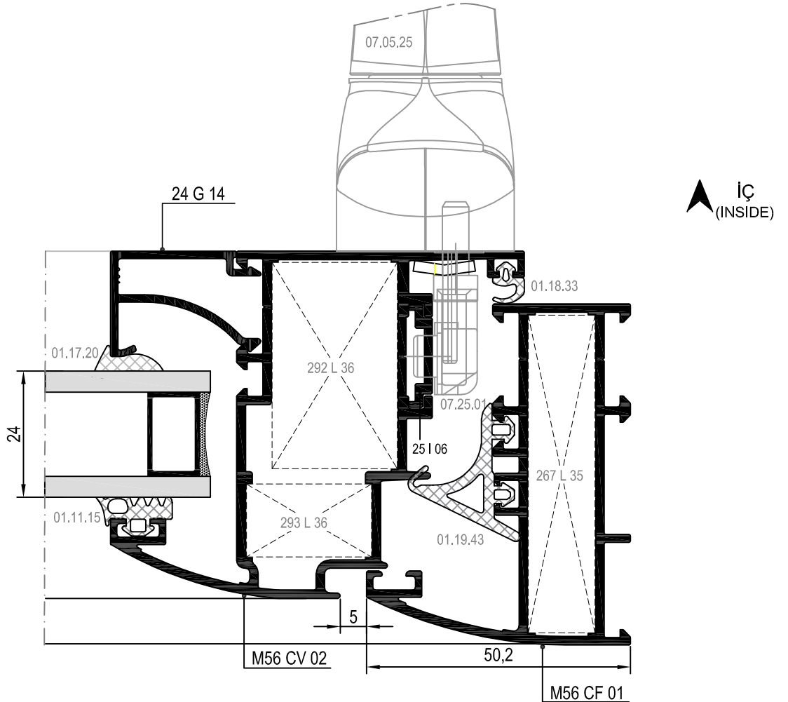
16 DETAYI DETAIL
